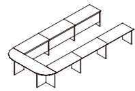
EU71-2 W4800•D2400•H760(mm)
