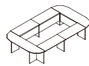
EU71-2 W4000•D2400•H760(mm)
